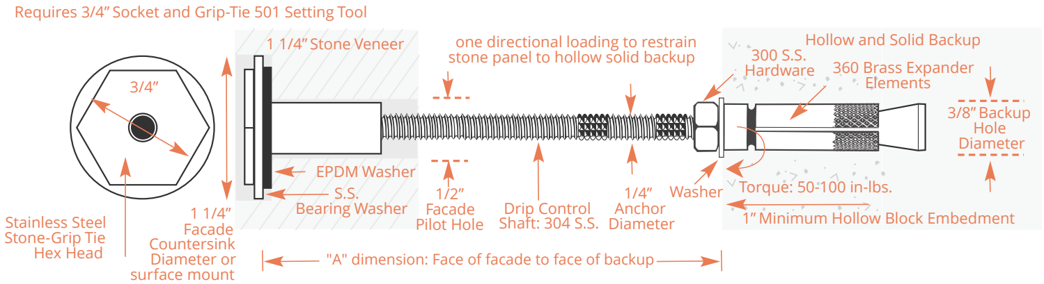
Type 1: Wind load restraint for one direction loading to hollow and solid back-up.
