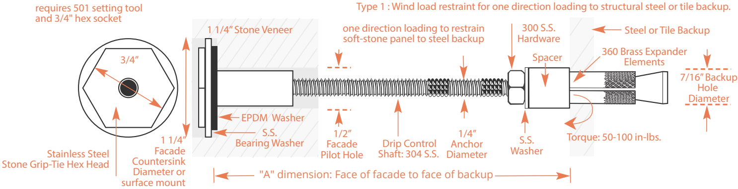
Type 1 : Wind load restraint for one direction loading to structural steel or tile backup.
