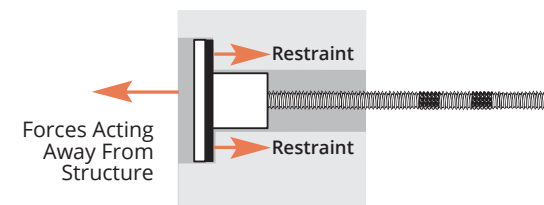
Type 1 Wind load restraint for one direction (i.e. suction or movement away from the structure) loading.
