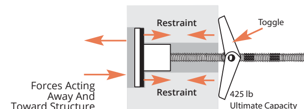
Type 2LD Light-duty wind load restraint for dual direction (i.e. suction and compression wind effects) loading.
