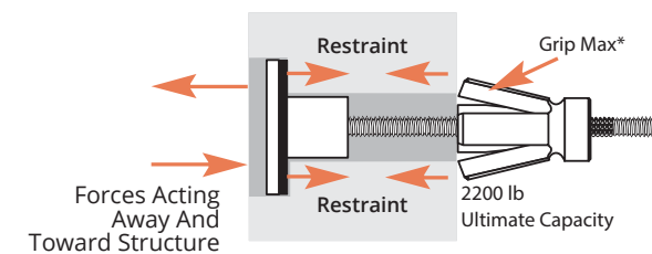
Type 2 Wind load restraint for dual direction (i.e. suction and compression wind effects) loading.
