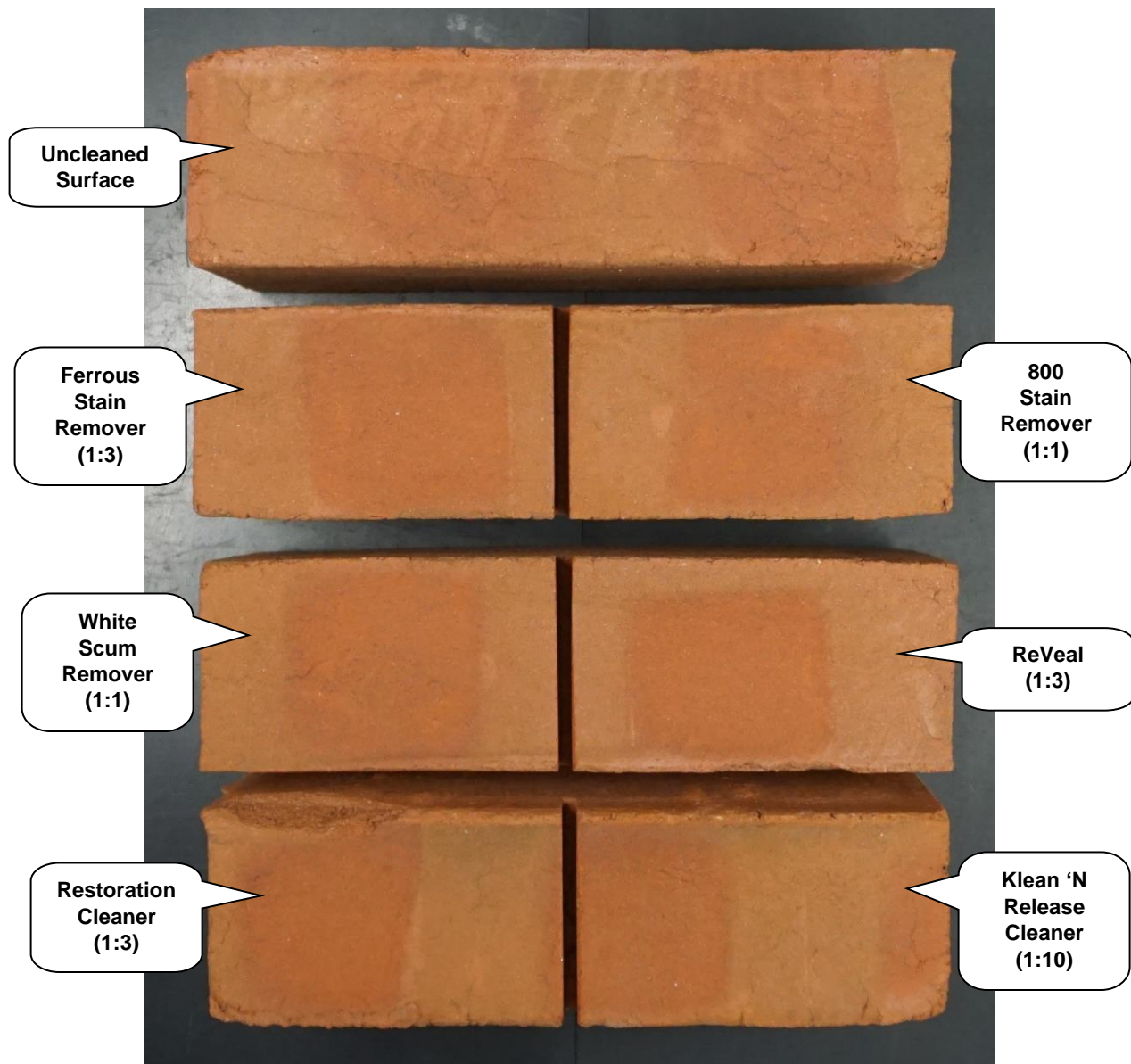
"53-DD" Facebrick After Cleaning
