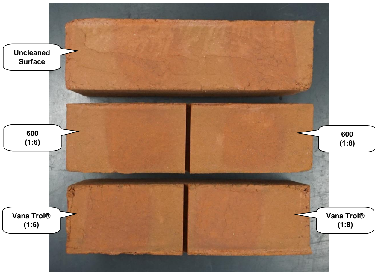
"53-DD" Facebrick After Cleaning
