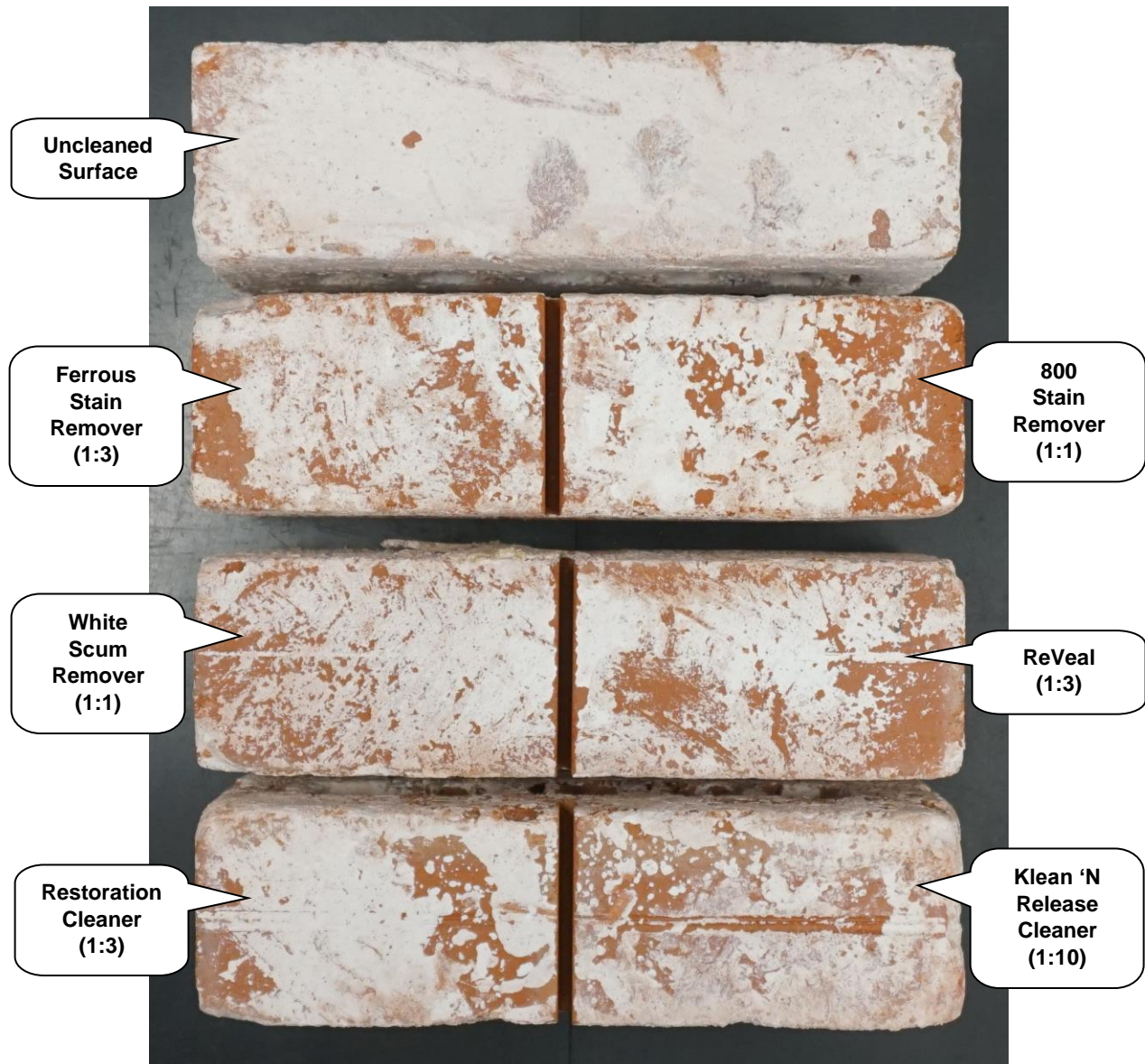
"Olde City" Facebrick After Cleaning
