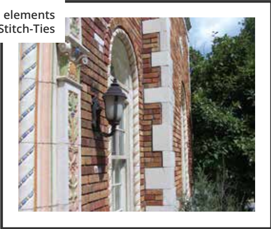
Re-anchoring to metal stud with CTP Stitch-Ties
