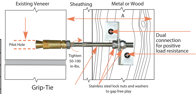
Grip-Tie Connection
